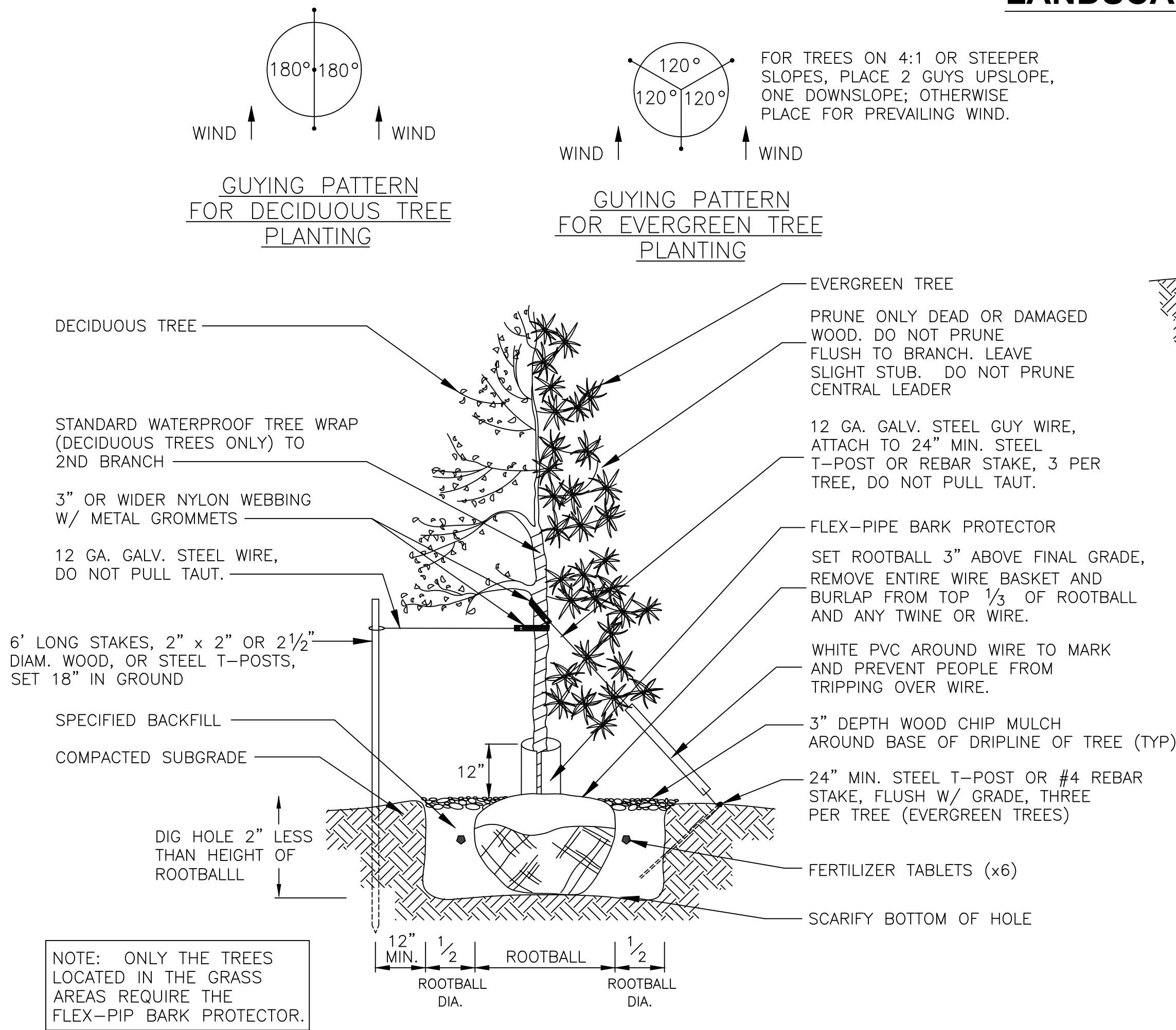
A TREE PLANTING SECTION L-3 NOT TO SCALE
